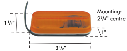
Replacement Lens MLR1030A (amber), MLR1030R (red) Replacement Bulb HB194
