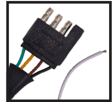
4-Way Flat Connector +wire for backup light
