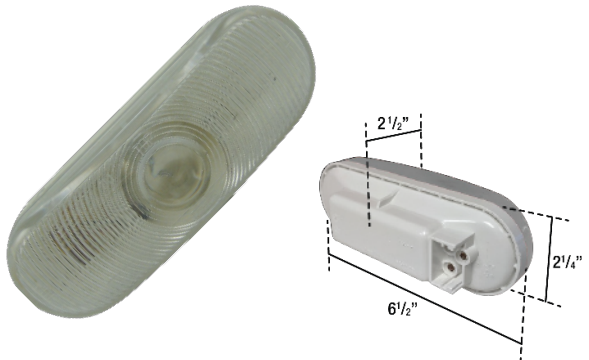
6" Oval Incandescent Series 12V Sealed Polycarbonate Lens & Base
