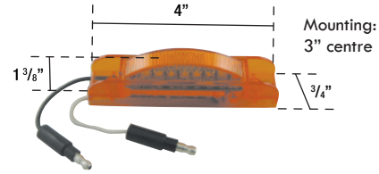
Female Bullet Connectors PT2022, PT2022-100R
